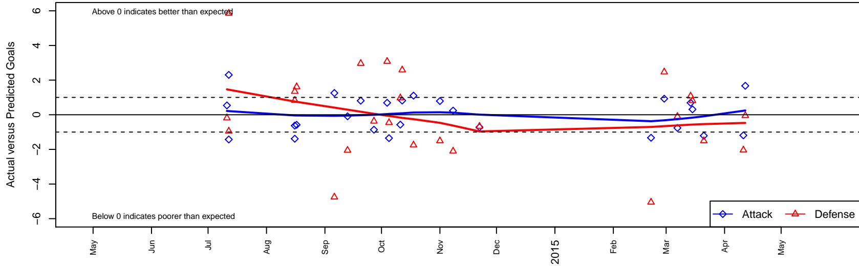
FC Tacoma White B03 Dots are actual minus expected GF (blue circles) and GA (red triangles). Blue line is smoothed change in attack strength. Red is smoothed change in defense strength.
